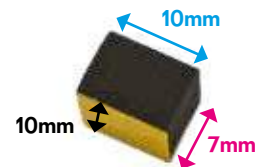
VB4000310 CALE VITRAGE H7 Megane II (02-08), Megane III CC (96-02)
